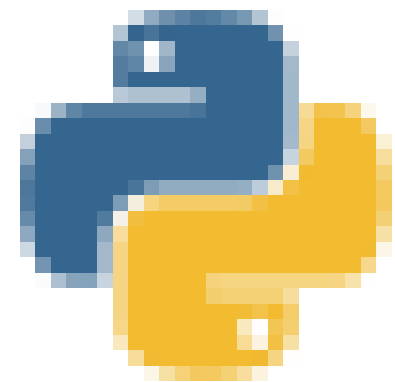
Python
